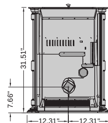
Back View
